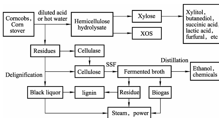
Fig.1 Corncobs or corn stalks biorefinery process schematic diagram
